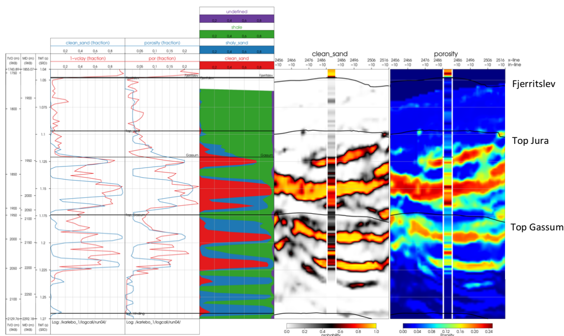
Figure 4 Lithology and porosity results predicted from the seismic inversion and projected on Karlebo-1A. First panel is showing seismic predicted probability of a clean sand (blue curve) and volume of clay from well log reversed (red curve). Second panel is showing seismic predicted total porosity (blue curve) and porosity from the well log (red curve). Third panel are showing the probability of the different lithologies based on the seismic inversion. Fourth panel is showing seismic predicted clean sand at a mini-section crossing the well log. The Fifth panel is showing the seismic predicted porosity at a mini-section crossing the well log.
