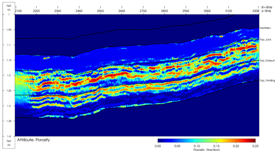
Figure 5 Total porosity estimated from the inversion and the lithology classification at line number 1.
