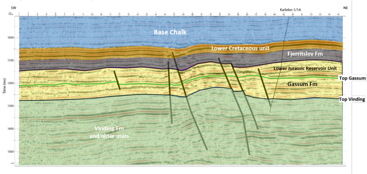
Figure 2 A geological interpretation in Two-Way-Time (TWT) of the main geological formations based on the seismic line number 5, about 7 km in length. The Karlebo-1A well path is projected on top. Extracted from Bredesen et al. (2019).
